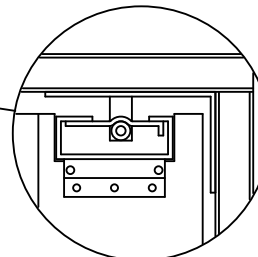
GS-HINGE ASSEMBLY
